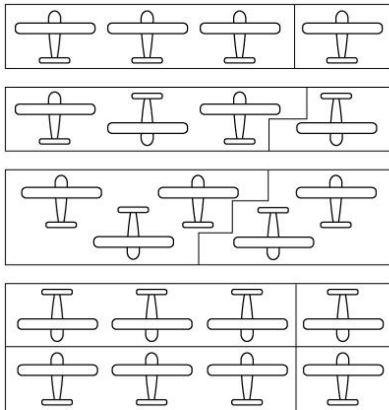
FIGURE A.4.1.3(b) Typical Configurations of Row Hangars.
